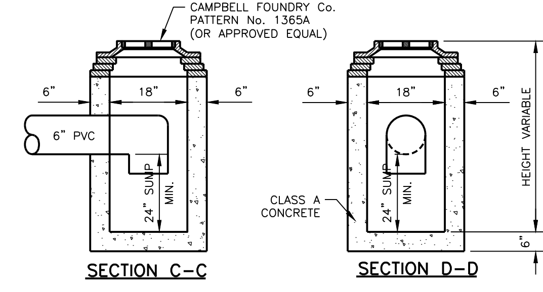
YARD DRAIN N.T.S.
