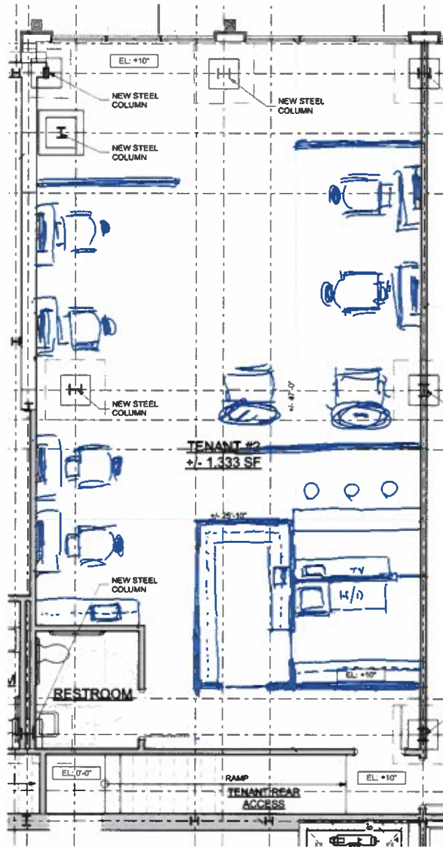
1 FIRST FLOOR SCALE: 1/4" = 1'-0"
